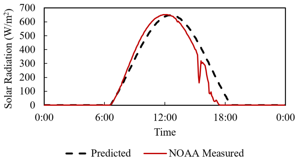
Figure 4.18 - Predicted vs. measured solar radiation in Fayetteville, AR - October 28, 2015
