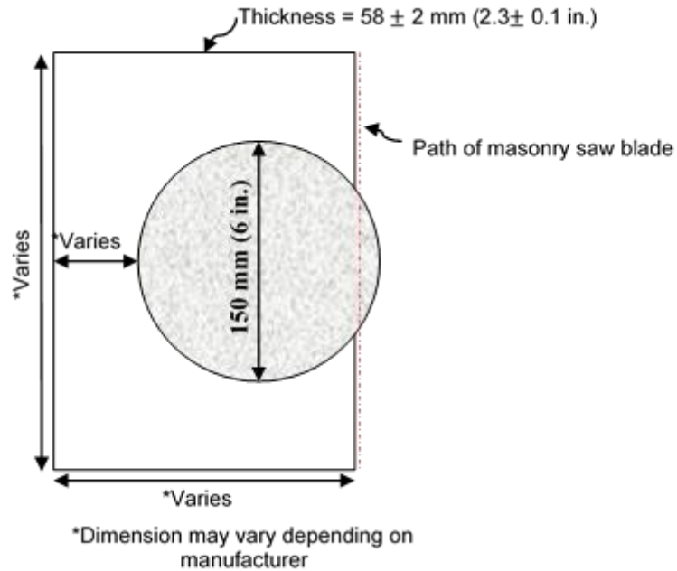
Figure 5: Sample-trimming process
