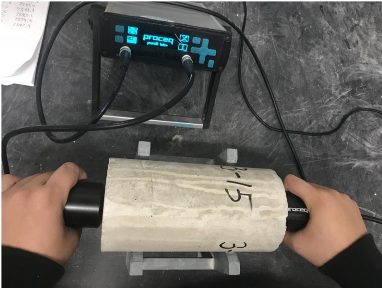
Figure 3-6: Experimental setup for ultrasonic pulse velocity test
