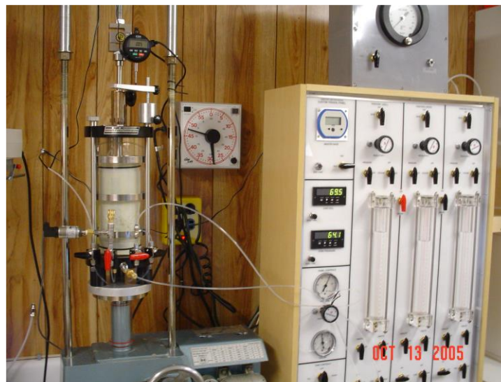
Figure 54. Shear Stage of Triaxial Test on Clay Specimen (Gregory 2006)
